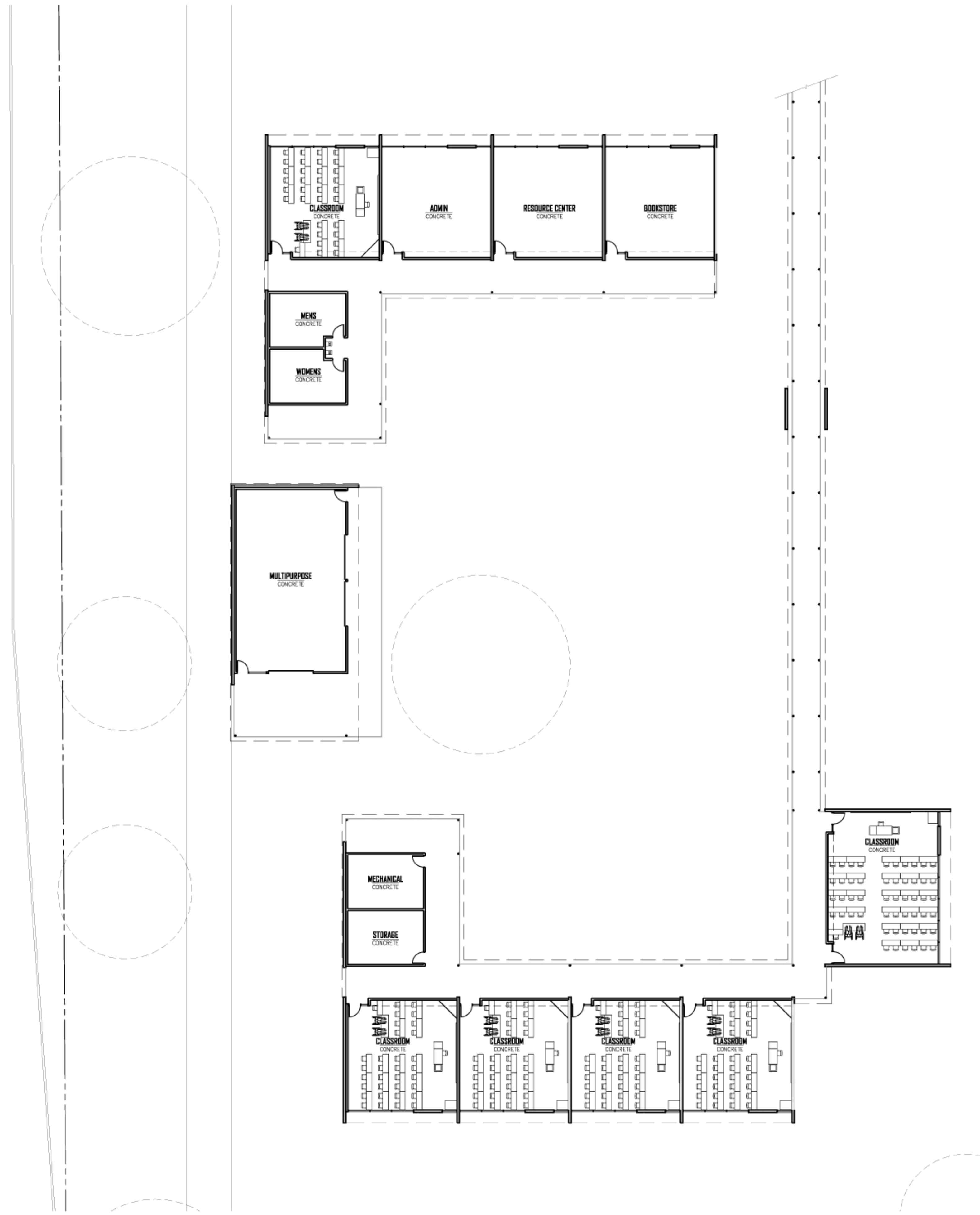
1 FIRST LEVEL PLAN 1/16"=1'-0"
